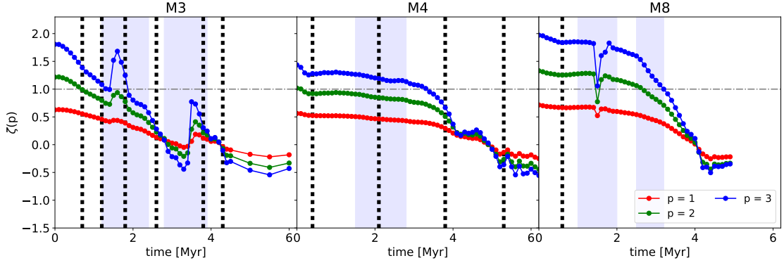
Figure 4.2: Time evolution of scaling exponent \zeta of the p^{\text{th}} order structure function in M3 ( left ), M4 ( middle ), and M8 ( right ). The black dotted lines indicate the times when SNe occur, and the blue shaded areas do so when mass accretion peaks within the respective clouds.
