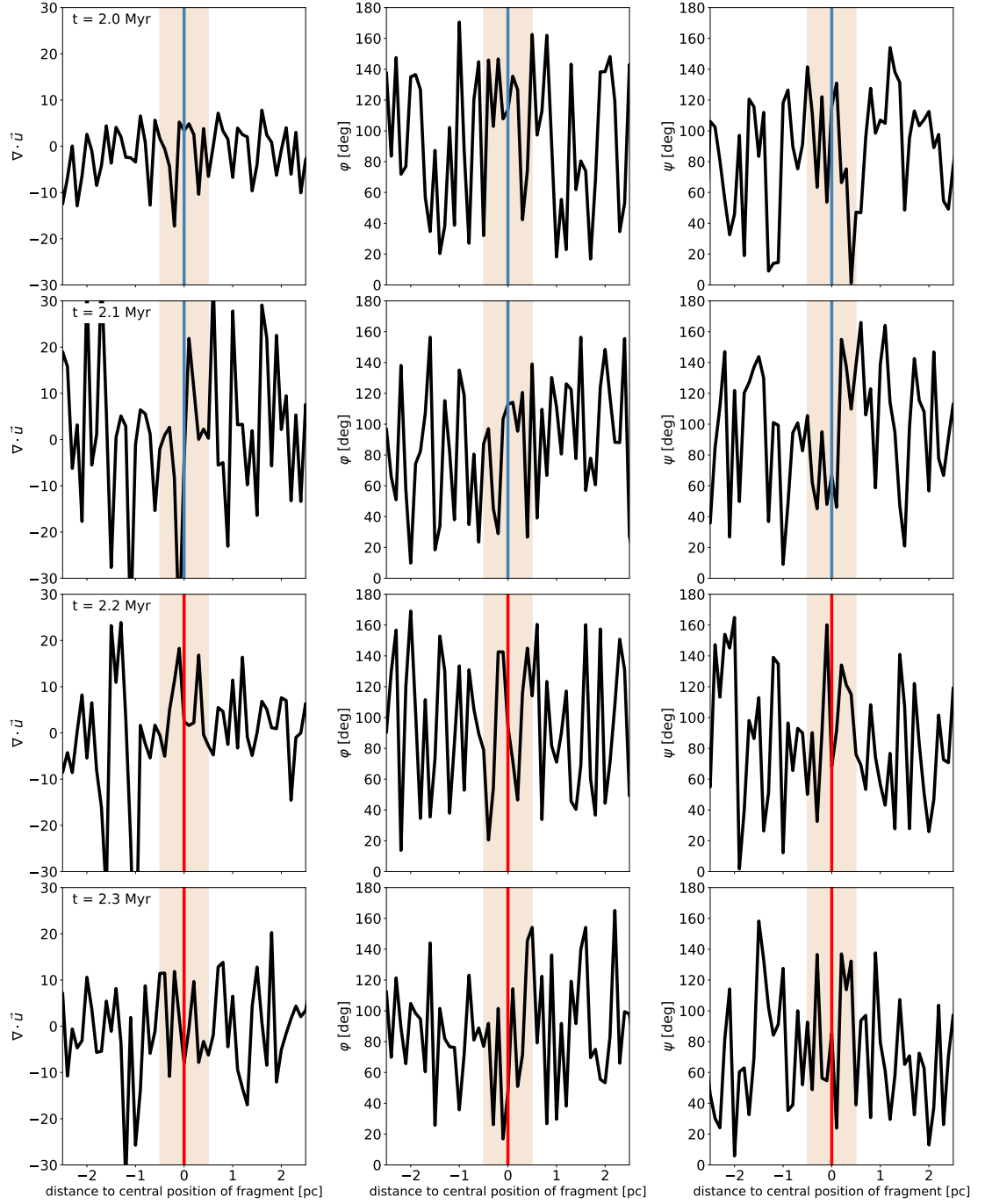
Figure 4.12: Zoom on fragment M4_f001 within t = 2.0\text{--}2.3 Myr (from top to bottom ). Shown are the measured values of \nabla \cdot \vec{u} ( left ), \phi ( middle ), and \psi ( right ) along the filament M4#001 at the given time steps. The abscissa refers to individual segments of the filament at the given distance to the central position of the fragment of interest. The orange area illustrate the radius of the fragment. The blue vertical lines mark the future position of the not-yet formed fragment, whereas red vertical lines indicate the actual position.
