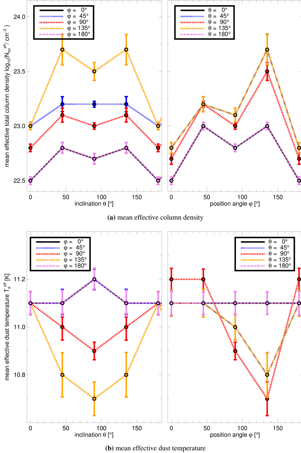
Figure 2.8: \rho Ophiuchi cloud model. The plots show the mean values of the effective total column density PDFs, \bar{N}_{\text{tot}}^{\text{eff}} (top), and effect dust temperature, \bar{T}_d^{\text{eff}} (bottom), as a function of the inclination, \theta , and position angle, \phi . The error bars illustrate 1\sigma errors. Note that I only show the values for inclinations \theta \leq 180^\circ because the values for \theta and \theta+180^\circ are identical.
