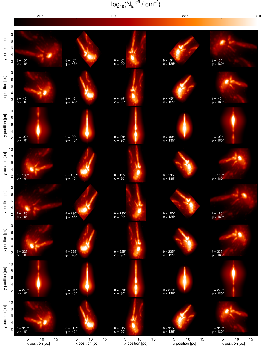
Figure 2.6: \rho Ophiuchi cloud model. As Fig. 2.5 showing the effective total column density along the LoS, N_{\text{tot}}^{\text{eff}} .
