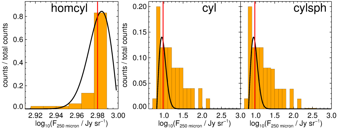
Figure 2.2: Probability density functions (PDFs) showing the 250\ \mu\text{m} flux density, F_{250\mu\text{m}} . From left to right, the plots show the PDFs of the homcyl , cyl , and cylsph models, all at (\theta, \varphi) = (0^\circ, 0^\circ) and T_{\text{iso}} = 10\ \text{K} . The black lines show the Rayleigh distributions fitted to the PDFs. The fitted mean values are marked with red lines.
