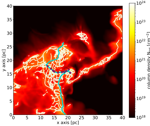
Figure 3.6: Column density map of M3 at t = 3.8 Myr when projected along the z axis with filaments identified using the 3D low density threshold of 100 \text{ cm}^{-3} (projected, white lines ), and the 3D high density threshold at 5,000 \text{ cm}^{-3} (projected, light blue lines ). The projected positions of identified density fragments are shown with purple dots.
