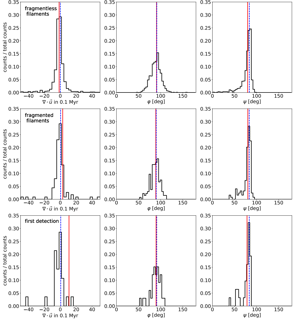
Figure 4.9: Histograms of 3D velocity divergence, \nabla \cdot \vec{u} (left), the angles between the filament skeletons and velocity vectors, \phi (middle), and angles between neighbouring velocity vectors, \psi (right). The individual counts represent the measured mean value of an entire filament that does not or does inhabit any fragment (top and middle, respectively). The histogram in the bottom panel illustrates the measurements of fragmented filaments at the very time step when a new fragment has been detected. The solid red lines and blue dashed lines mark the mean and median values, respectively.
