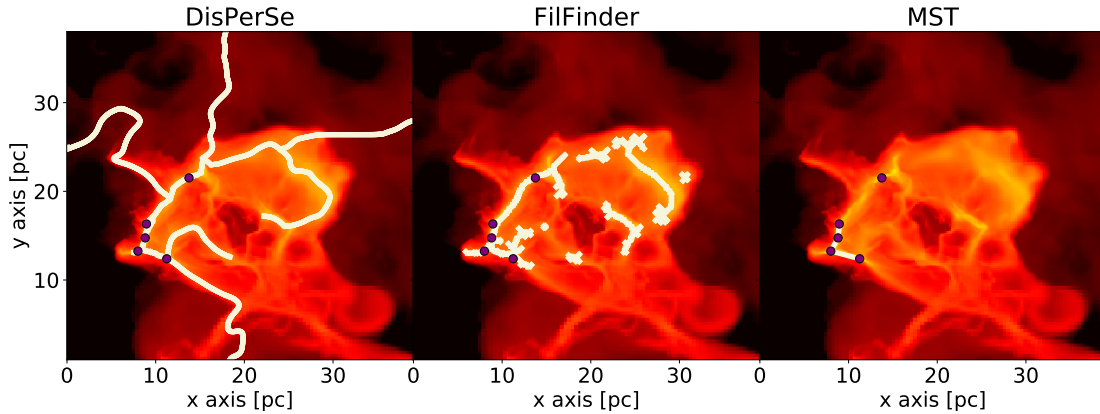
Figure 3.2: Example for structures identified by DisPerSe ( left ), FilFinder ( middle ), and MST applied to fragments from astrodendro ( right ). The background shows the column density map of M4 at t = 2.7 Myr along the z axis, ranging between 10^{18} to 10^{24} \text{ cm}^{-2} . The purple dots represent the position of cores identified by astrodendro. The white lines illustrate filamentary structures found by the three filament finders, applying a column density cut at N_{\text{th}} = 1.5 \times 10^{21} \text{ cm}^{-2} .
