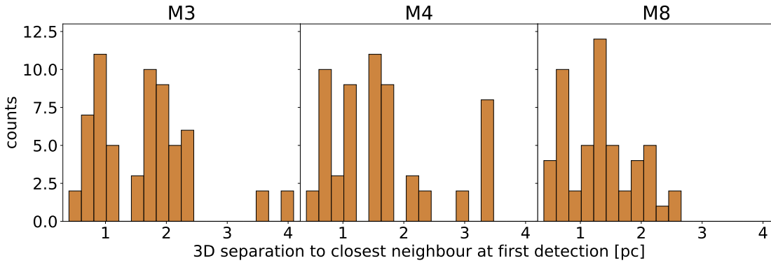
Figure 3.15: Histogram of separations of fragments within M3 ( left ), M4 ( middle ), and M8 ( right ) to their closest neighbour at the time when the fragment was detected for the first time.
